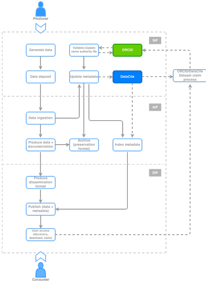
UKDA workflow for new data
