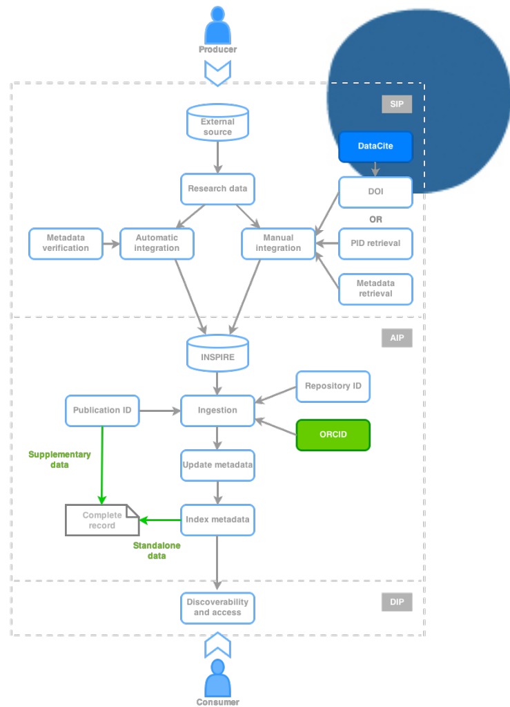
INSPIRE workflow for current data
